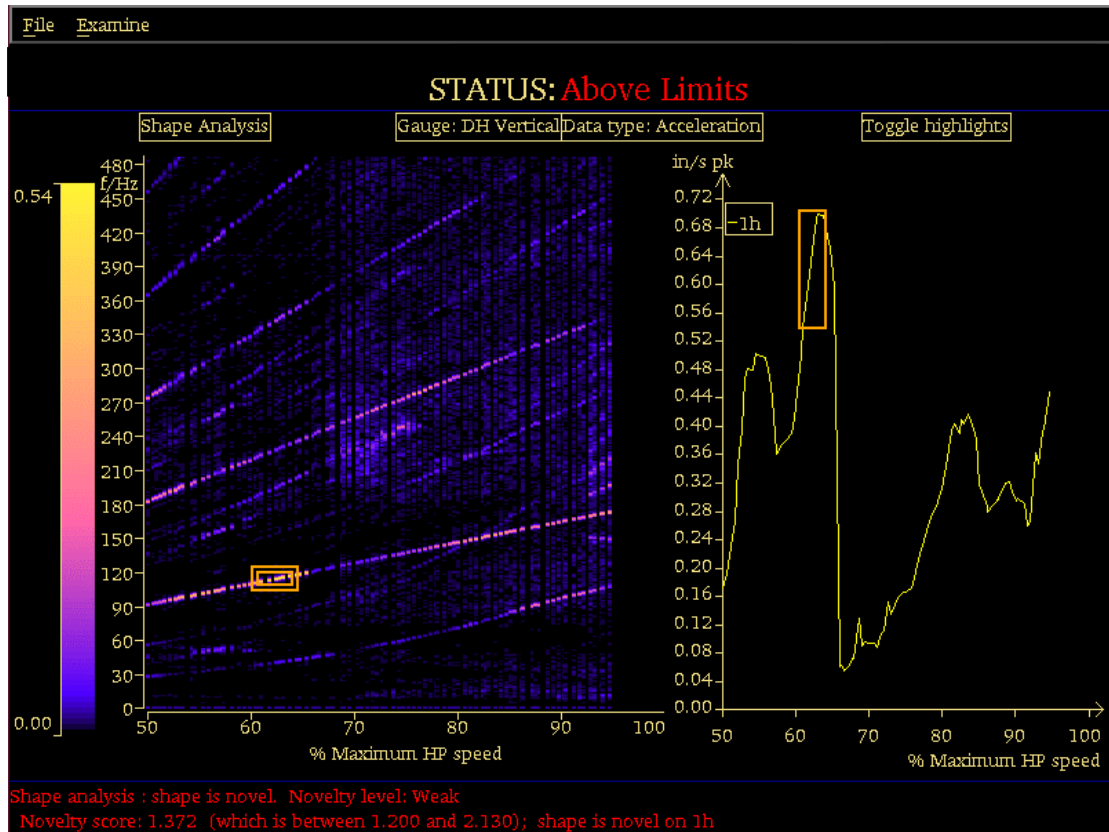
Figure 1. Typical engine vibration data captured by the QUOTE system. On the left is a plot of vibration against shaft speed. The graph shows a box where there is an anomaly, expanded on the right. The right plot shows one ‘tracked order’ and the same anomaly as indicated on the left.
