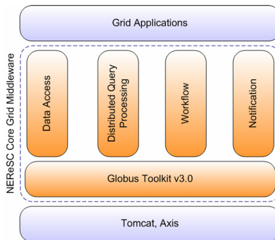
Figure 5: The initial release of the NEReSC Core Grid Middleware
