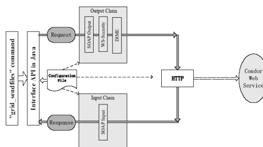
Figure 1: Message filter chains.
