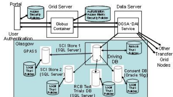
Figure 4: VOTES Architecture
